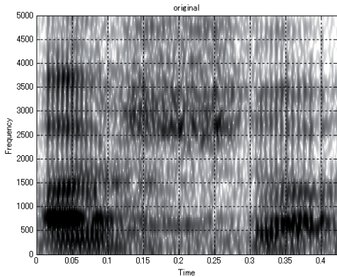
Figure 2. Target /a/ utterance produced by subject FH.
