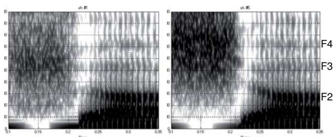
Figure 6. Spectrograms of synthesized /a/ sequences ([ʃa] transition shown). /a/ length = 16 cm, ratio = 0.9. Left: 'apical' /ʃ/; right: 'palatalized' /ʃ/.
