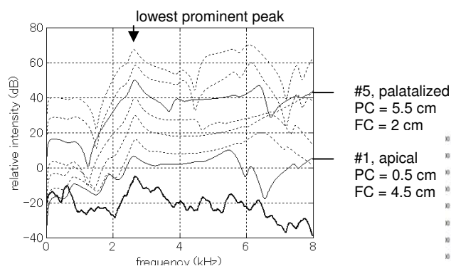
Figure 5. Time-averaged spectrum of /ʃ/ extracted from the target /a/ utterance (bottom thick line) and transfer functions (shifted by 20 dB) of /ʃ/ configurations giving rise to a lowest prominent peak close to that of the natural utterance. The palatal channel lengthens and the front cavity shortens from bottom to top.
